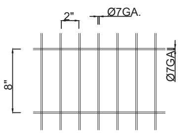
Mesh Detail
